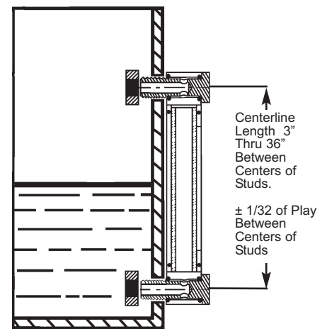
Typical Installation
