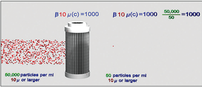
Hy-Pro G8 Dualglass media performance
