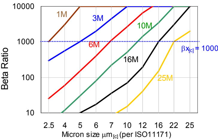
Glass Media Code Filtration Efficiency (Beta Ratio) vs Micron Size
